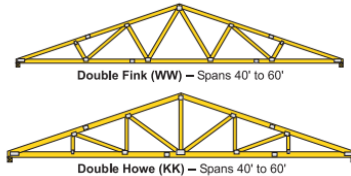
Fig5. Types of trusses
